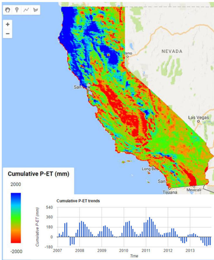
Figure 21: Cumulative P-ET (precipitation - evapotranspiration) in California (2007-2013).
