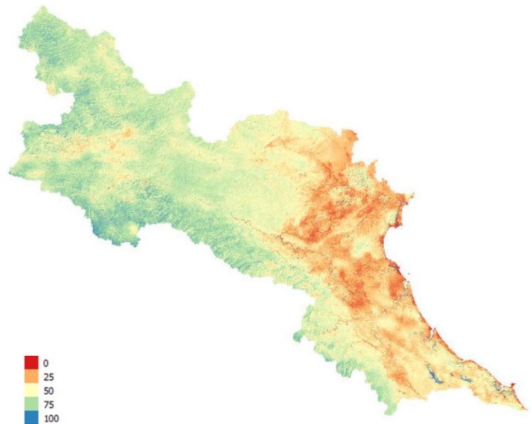
Figure 19: Downscaled ET for the Ca river basin in Vietnam (values in mm/month).
