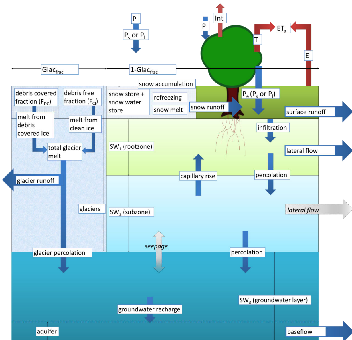
Figure 8: SPHY model concepts.
