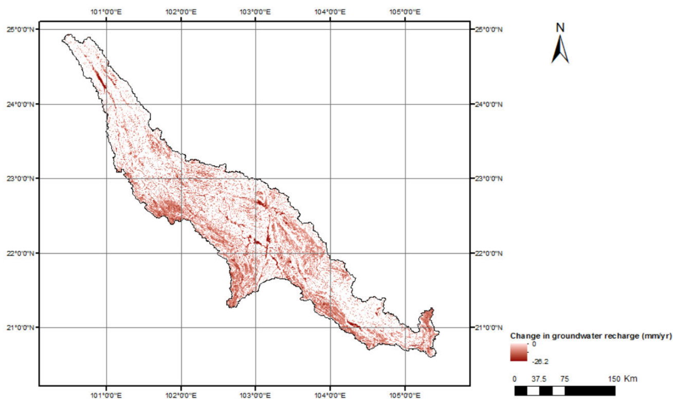
Figure 14: Predicted changes in groundwater recharge in the 2050s as compared to baseline conditions.
