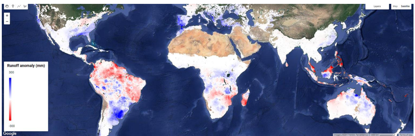
Figure 22: Global runoff anomaly in the El Nino year 2009 - 2010 for December until February computed with a preliminary version of the WaterPix model (Poortinga et al. , 2017).
