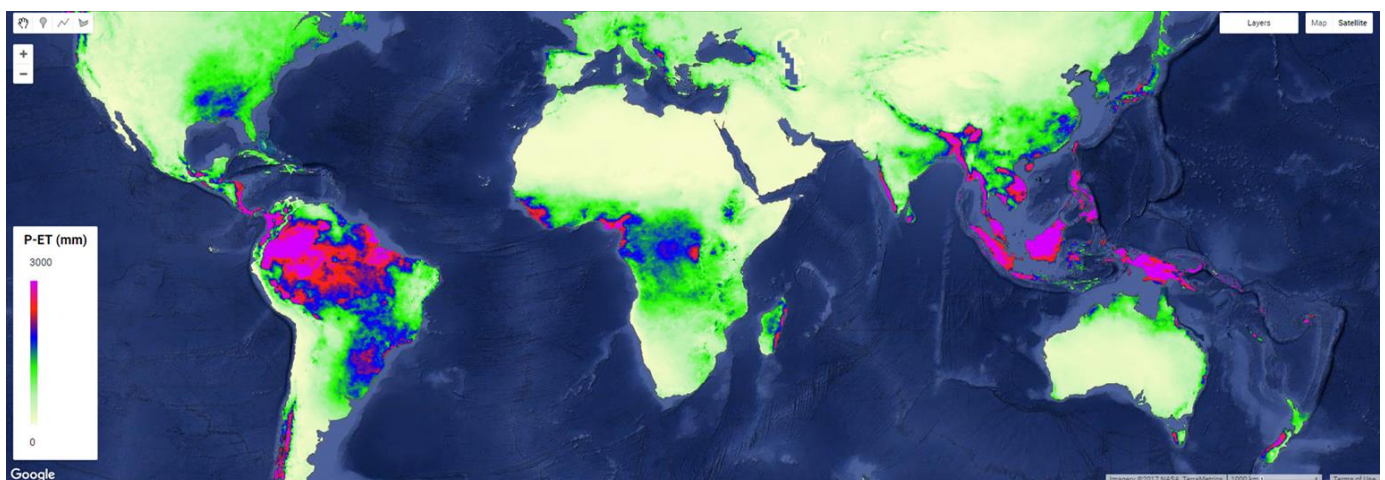
Figure 20: A global map of precipitation (P) minus Evapotranspiration (ET) for the year 2009. CHIRPS is used for P and MOD16 is used for ET.
