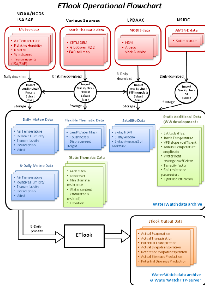
Figure 11: ETLook flowchart.
