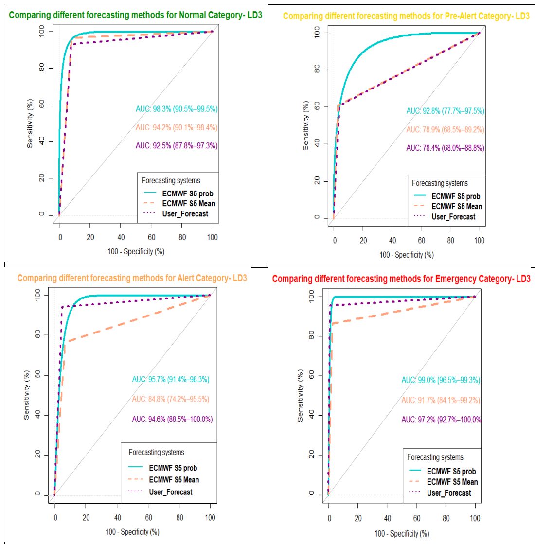
Figure 3-6: ROC curves for drought index predictability comparing all forecasting methods for lead time 3 (Mars, June, September and December) over the long period 1982-2010
