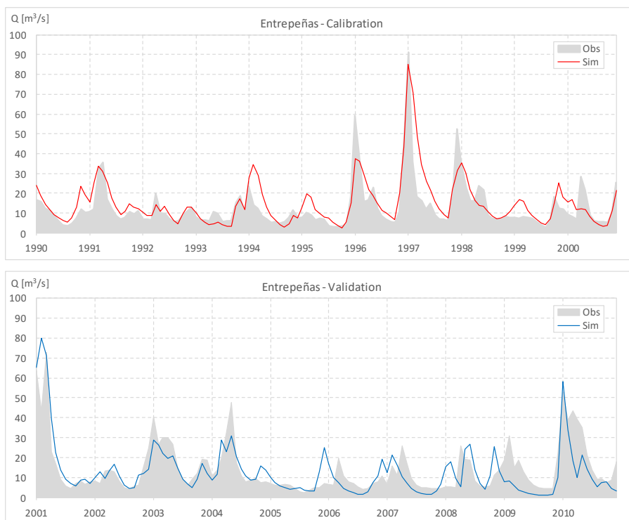
Figure 3-2: Hydrographs for station 1 (Entrepeñas), calibration (1990-2000) and validation (2001-2010) periods.
