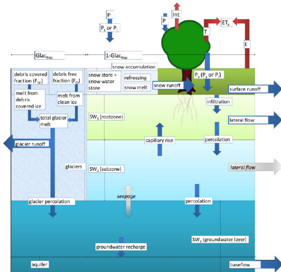
Figure 2-2: Conceptual scheme of the hydrological model SPHY
